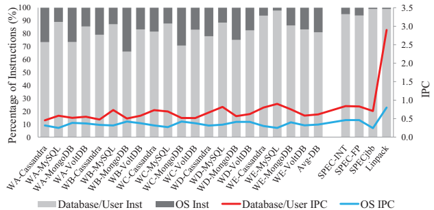
Fig. 3: Percentage breakdown of user/database and OS instructions for each workload
