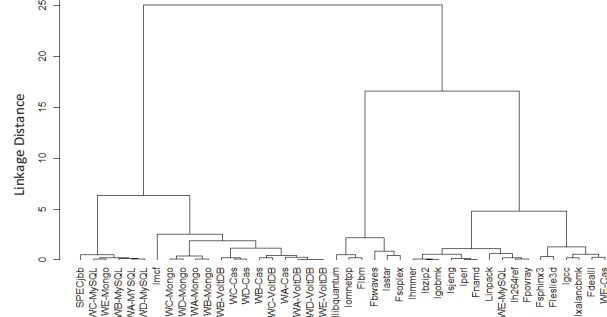
Fig. 10: Dendrogram comparing databases with SPEC, SPECjbb and Linpack benchmarks based on cache performance
