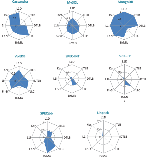
Fig. 12: Kiviat diagrams of the representative workloads. Database runs are for workload A. [Note the change of scale for Linpack]
