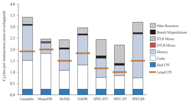
Fig. 9: Non-overlapped and Actual CPI for database workloads
